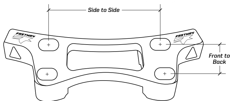
HAND GUARD TOP CLAMP MEASUREMENT GUIDE
